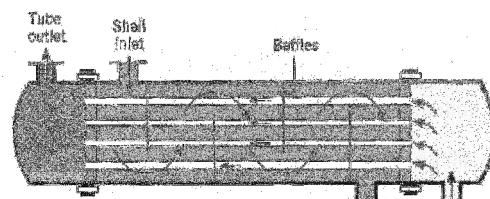
Shell-and-tube heat exchanger with one shell pass and one tube pass (cross-counterflow mode of operation).
