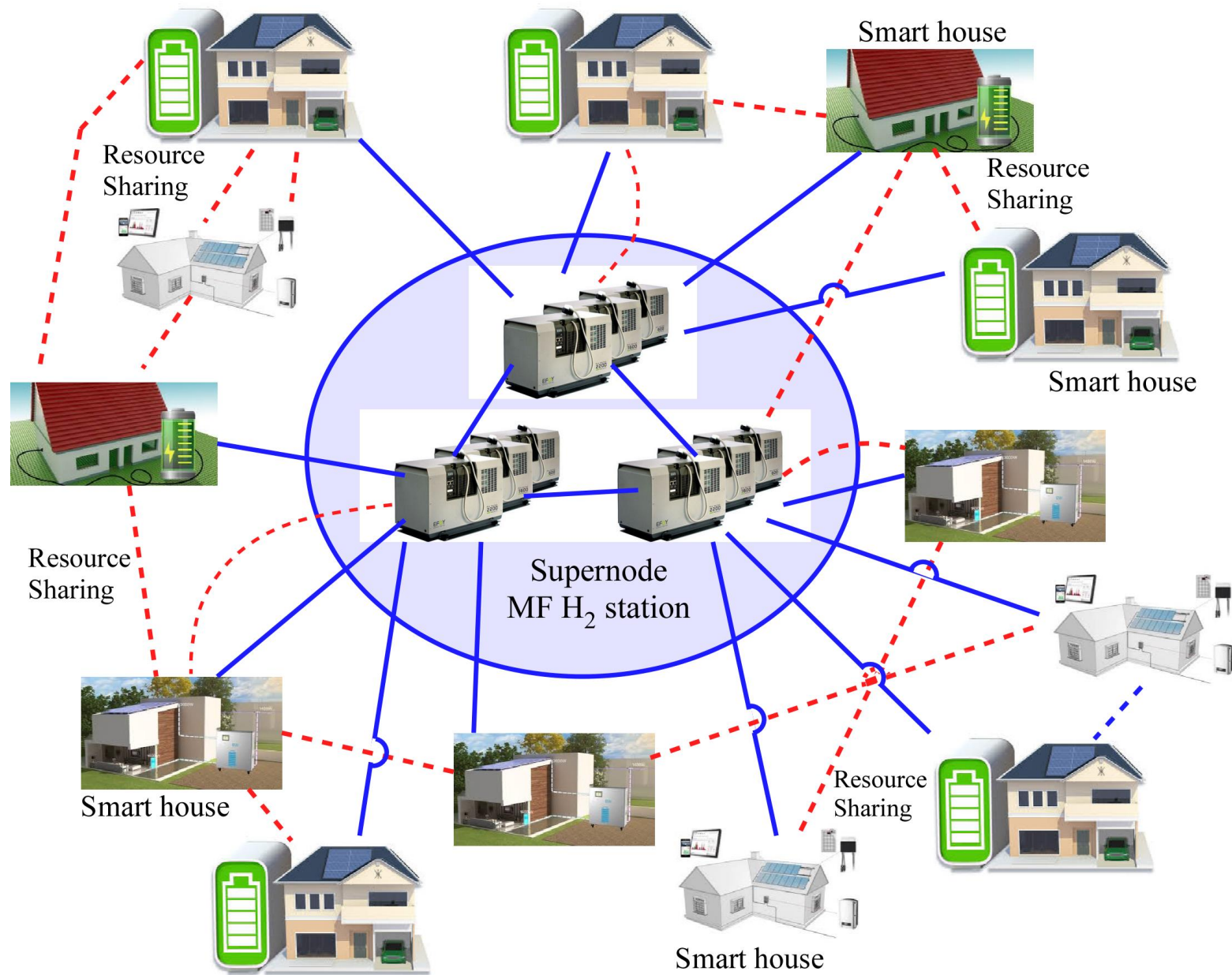
Example of peer-to-peer H 2 supply chain based on a 2-layered model.
