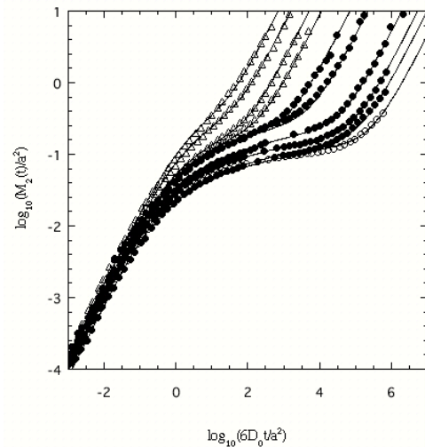
Figure 1: A log-log plot of the mean-square displacement vs time. Etc., ...
