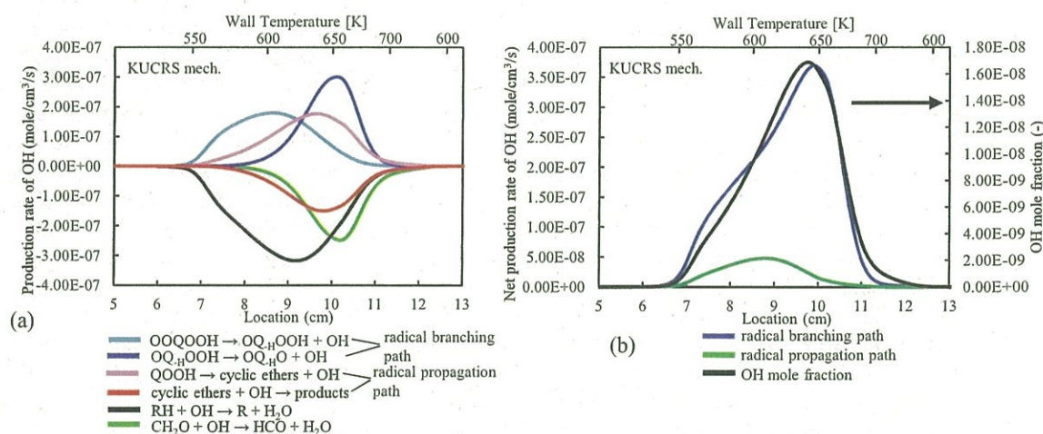
Fig. 3 Profiles of top three reactions in OH production and consumption (left : 3.a) and profiles of net rates of OH production by radical branching and propagation paths and OH mole fraction profiles from different reaction mechanisms (right : 3.b).
