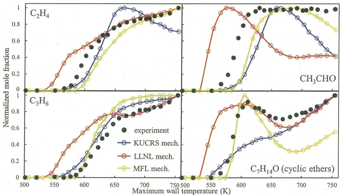
Fig. 5 Profiles of normalized mole fractions of representative species for radical branching path ( CH_3CHO ) and radical propagation path ( C_2H_4 , C_3H_6 and C_7H_{14}O ).
